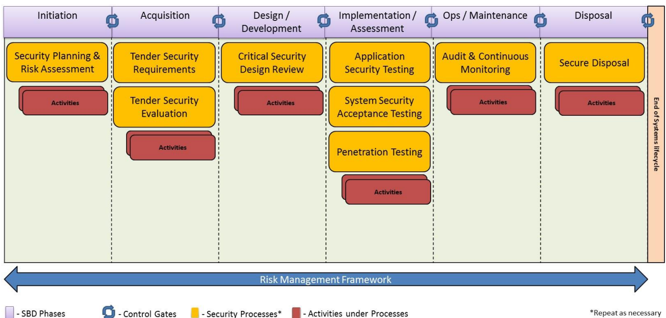
Figure 5: Security-by-Design Framework
